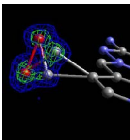
Figure 1. Three dimensional difference electron density map showing the disorder in the -CH 2 OH
