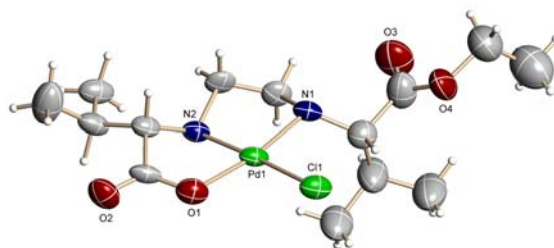
Figure 1. Structure of the complex
