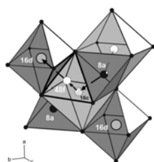
Fig.1: Crystal structure of \text{Li}_4\text{Ti}_5\text{O}_{12} .
