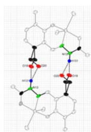
Figure 2. Packing in [Cu(PLSC)Cl 2 ] showing the disorder in the -CH 2 OH and the implications for the hydrogen
