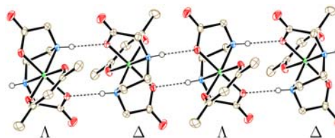
Fig. 2: Hydrogen bonds in s-cis -[Cr(edda)(acac)]
