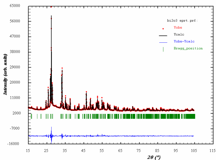
Figure 1. XRPD pattern after the refinement procedure using Rietveld's method
