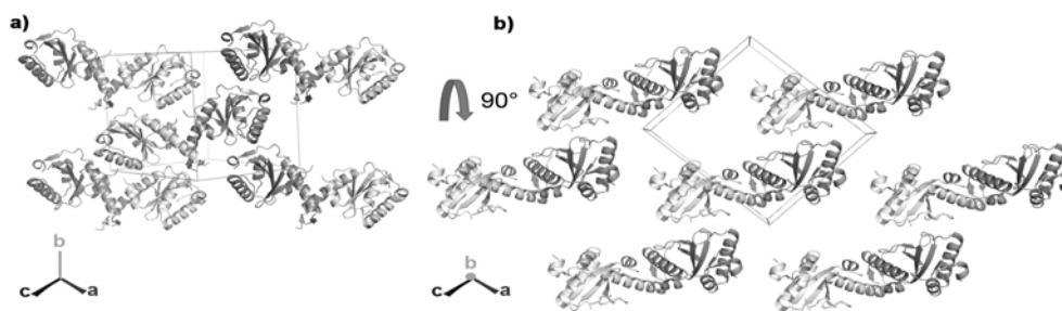
Crystal packing of the MjRelB – MjRelE protein complex in two projections
